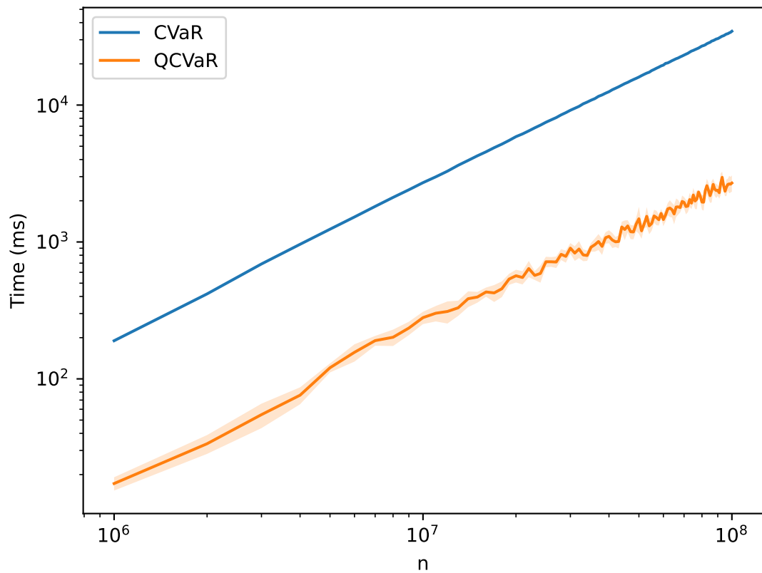
CVaR vs QCVaR
