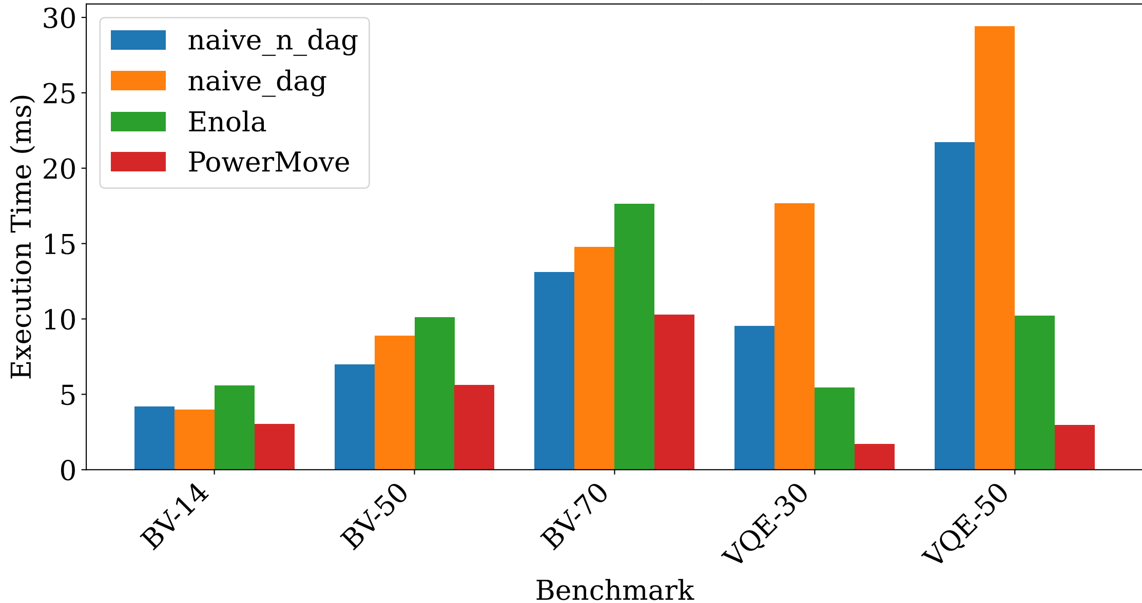
Execution Time: BV and VQE Benchmarks
