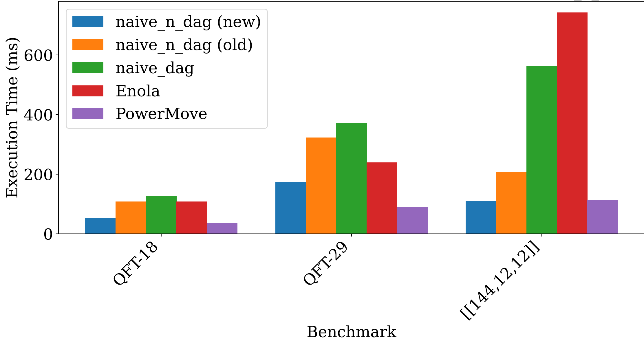
Execution Time: QFT and Other Benchmarks (New vs. Old naive_n_dag)
