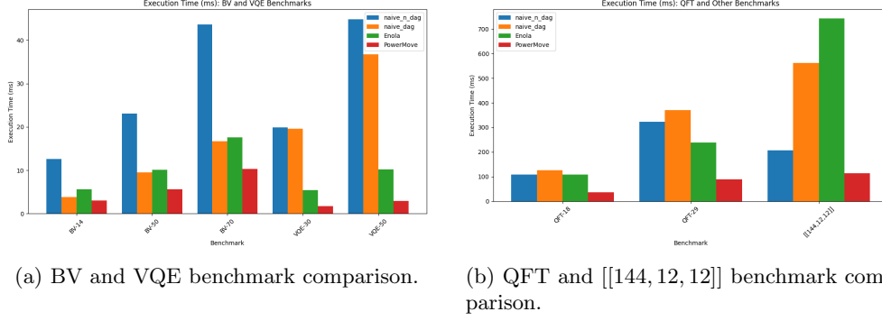
Fig. 5: Execution-time comparison across benchmark families for Enola, PowerMOVE, Naive_Dag, and Naive_N_Dag. The BV and VQE benchmarks test less regular or hub-like interaction patterns, while the QFT and [[144, 12, 12]] benchmarks contain more structured interaction patterns with greater potential for parallel execution.
