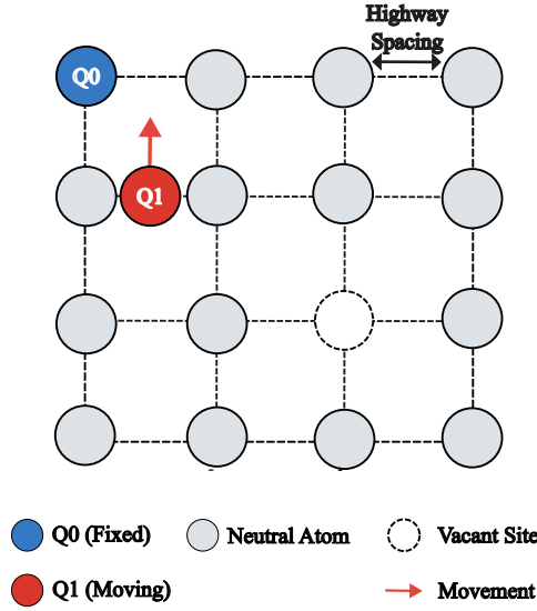
Fig. 1: Highway-based movement model for neutral-atom shuttling. The processor is represented as a two-dimensional array of trapping sites connected by horizontal and vertical movement highways. Occupied sites contain neutral atoms, while vacant sites provide available space for routing. In this example, qubit Q_0 remains fixed and qubit Q_1 is transported along the highway network until it reaches an interaction position near Q_0 . The highway spacing parameter controls the physical separation between neighboring movement lanes and helps maintain isolation between simultaneous two-qubit gate operations.
