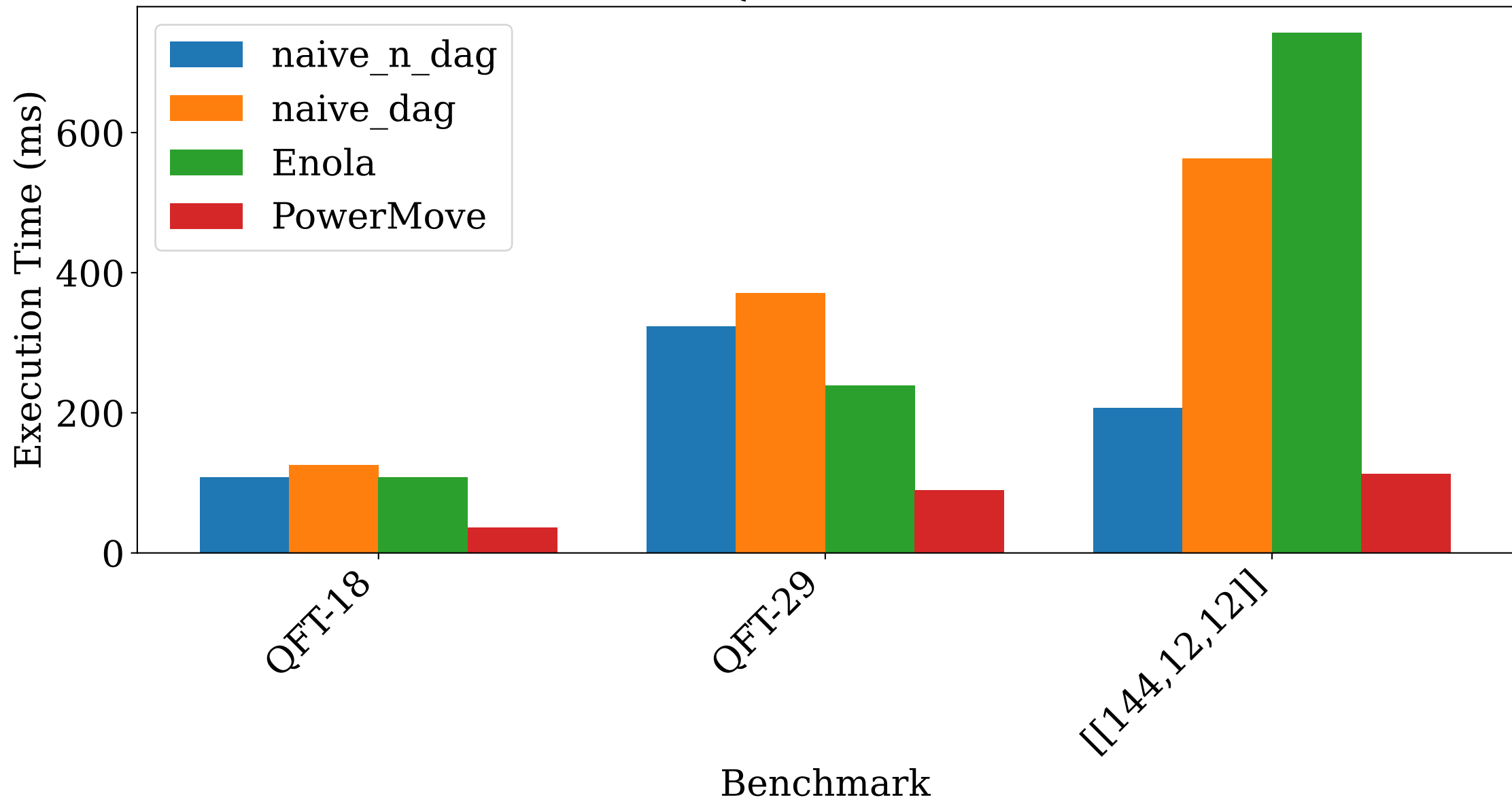
Execution Time: QFT and Other Benchmarks
