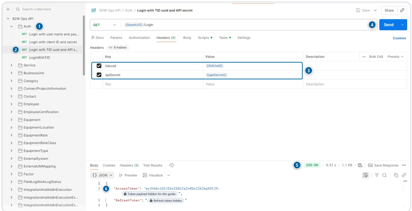
Figure 7. Generating a token. The numbers match the steps above. The token values are hidden.
