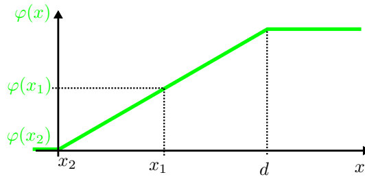
Figure 5.8: Representation of the potential curve \varphi(x) within the electric homogeneous field
