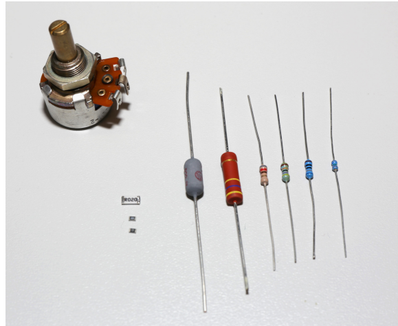
Figure 2.1: Different types of resistors. These include wirewound resistors, potentiometers and SMD resistors. The design and material determine the electrical properties, such as resistance value, load capacity and temperature coefficient.
