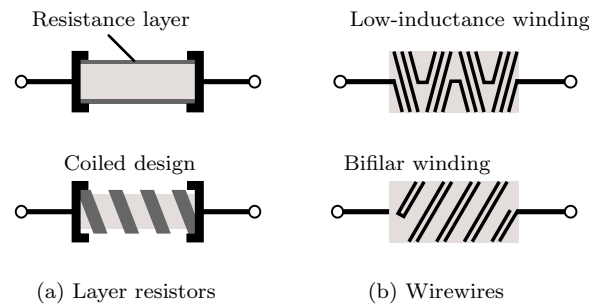
Figure 2.10: Various types of through-hole (THT) resistors.
