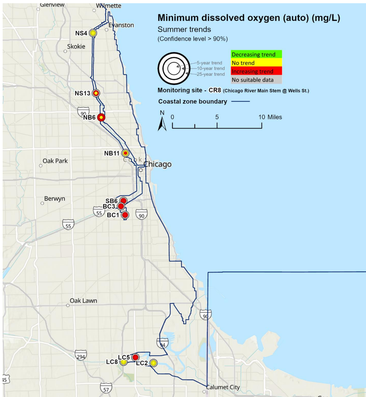
Summer trend slopes for minimum dissolved oxygen (mg/L per year)
