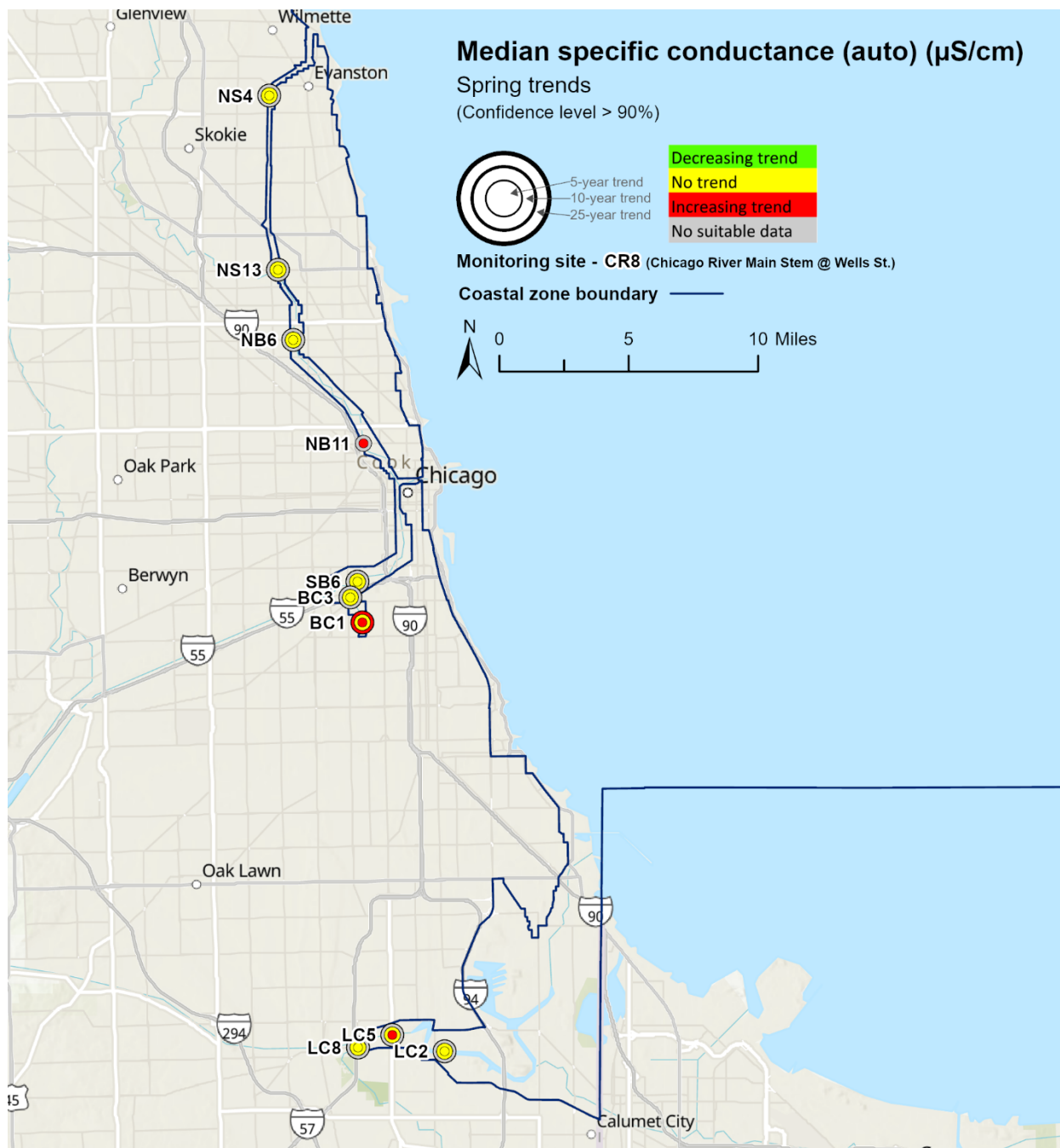
Spring trend slopes for median specific conductance ( \mu\text{S}/\text{cm} per year)
