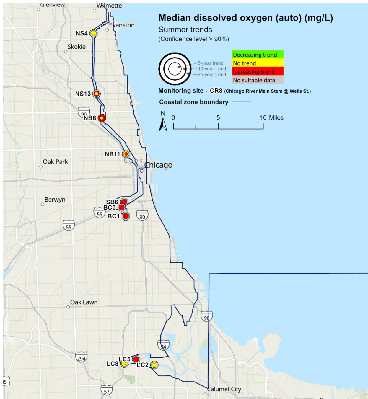
Summer trend slopes for median dissolved oxygen (mg/L per year)
