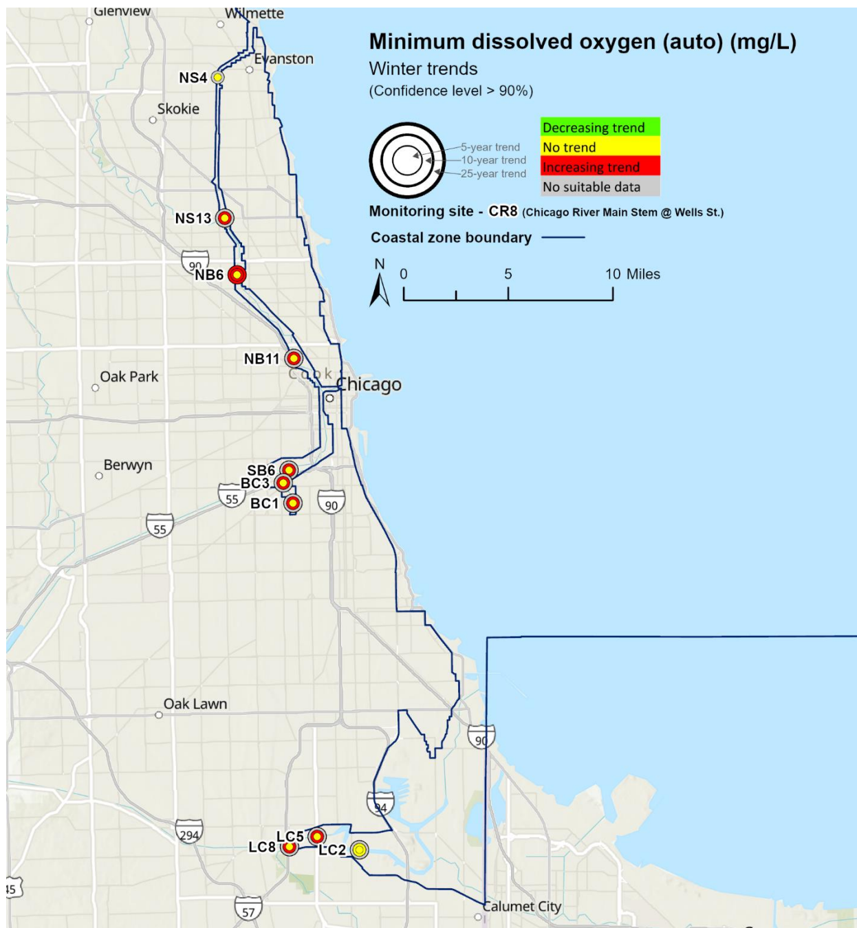
Winter trend slopes for minimum dissolved oxygen (mg/L per year)
