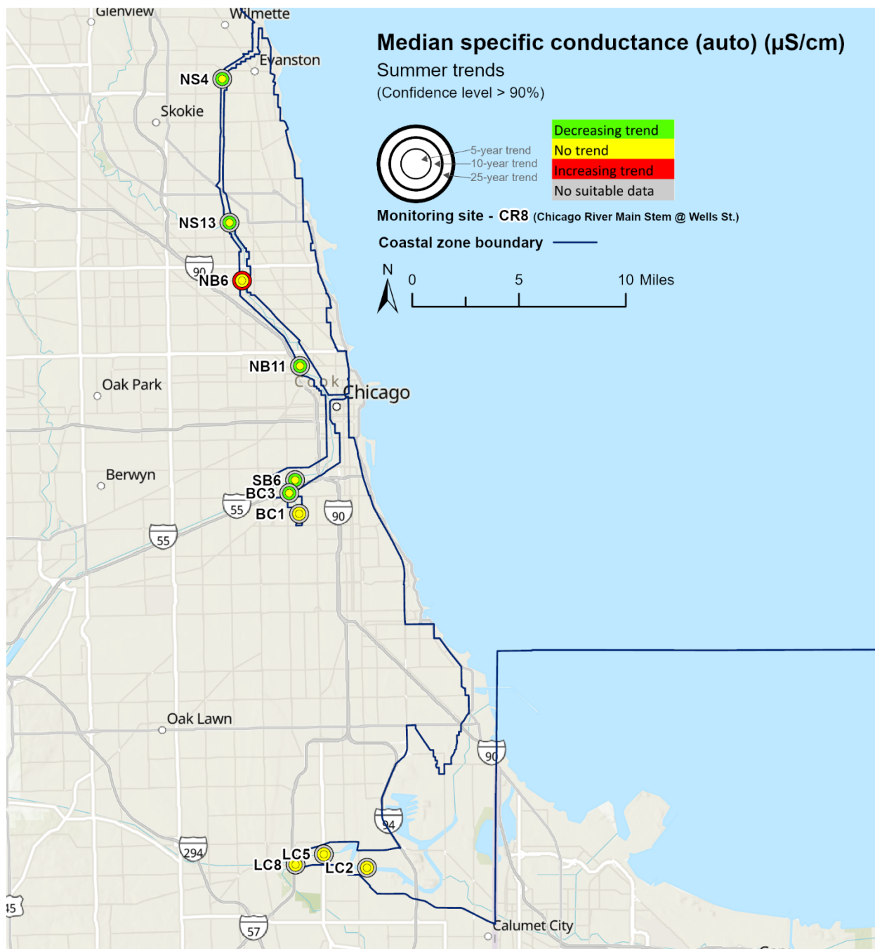
Summer trend slopes for median specific conductance ( \mu\text{S}/\text{cm} per year)
