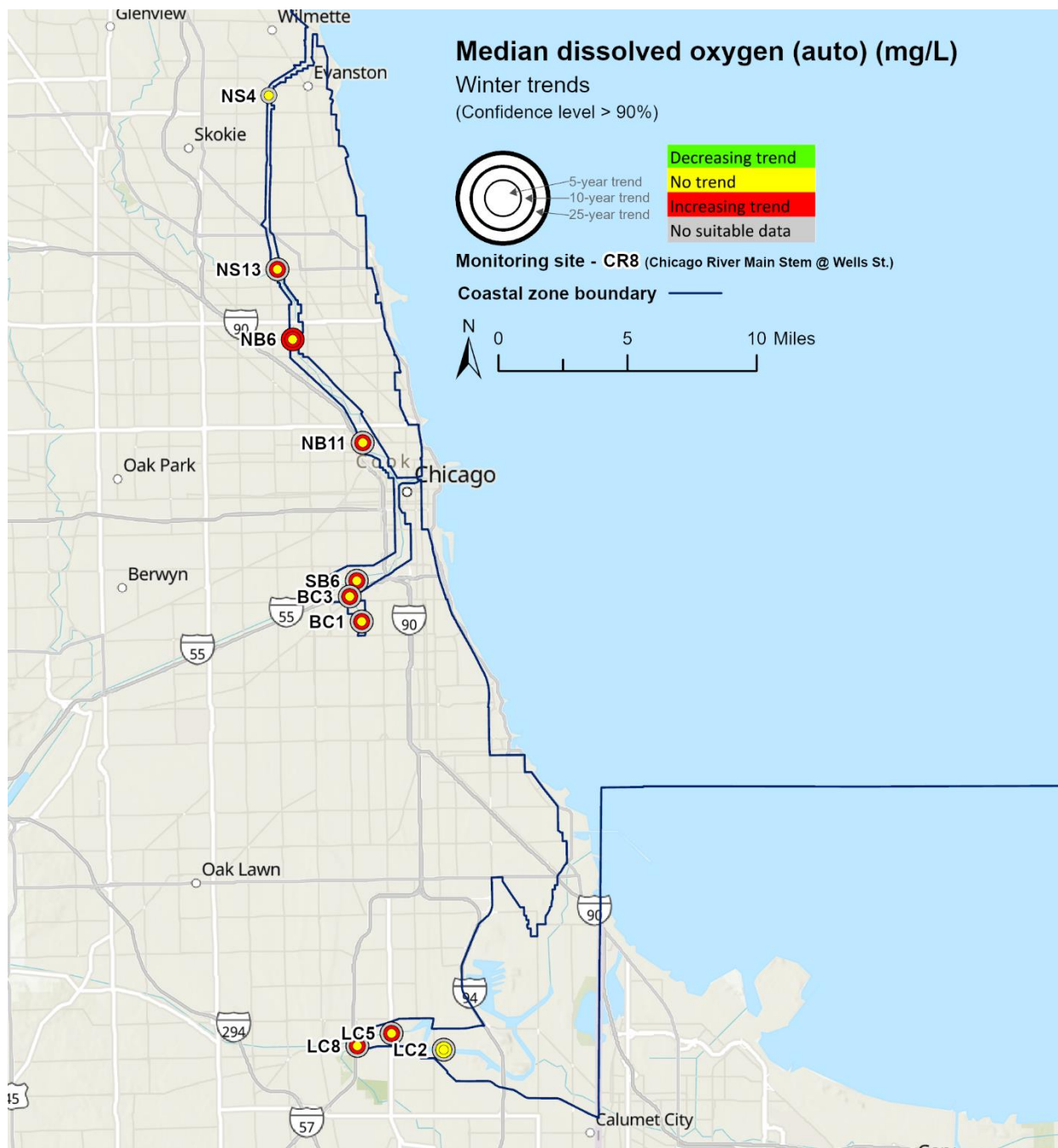
Winter trend slopes for median dissolved oxygen (mg/L per year)
