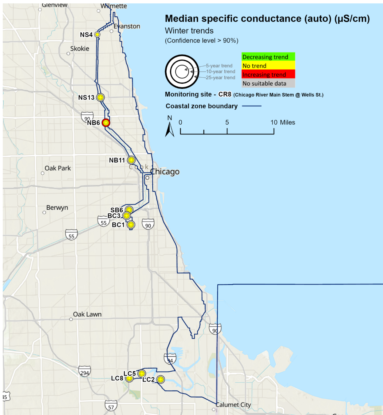
Winter trend slopes for median specific conductance ( \mu\text{S}/\text{cm} per year)
