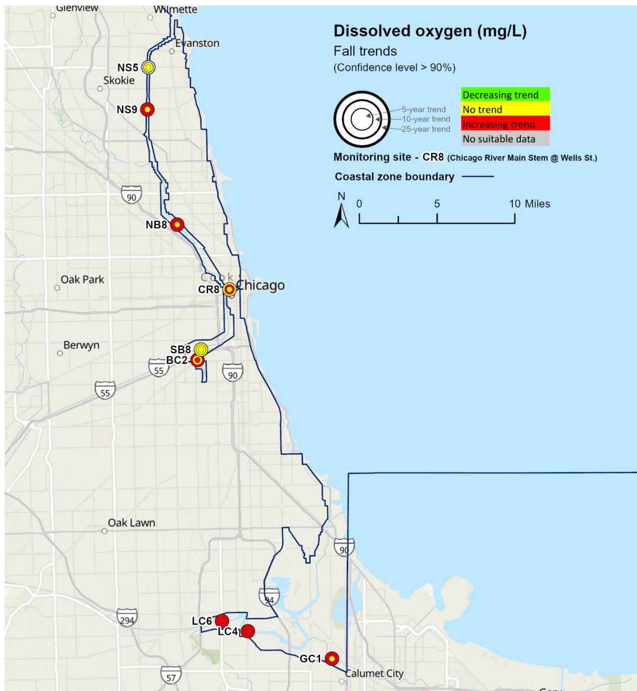
Fall trend slopes for dissolved oxygen (mg/L per year)
