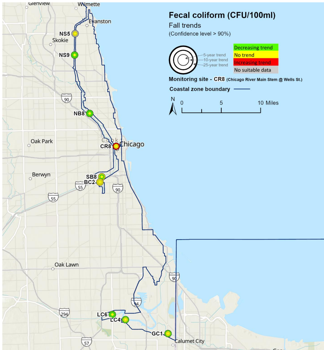
Fall trend slopes for fecal coliform (CFU/100mL per year)
