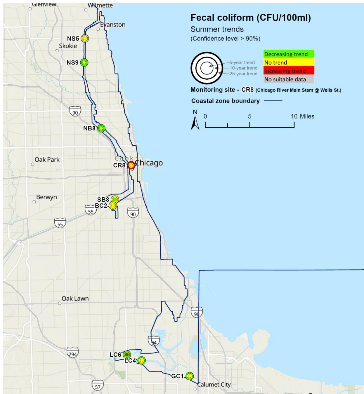
Summer trend slopes for fecal coliform (CFU/100mL per year)
