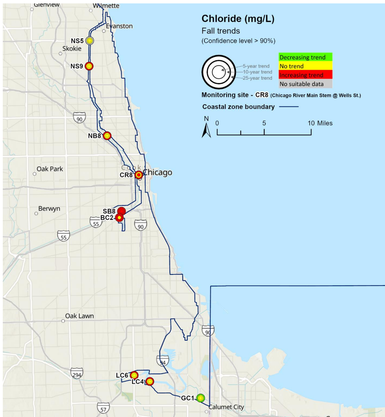
Fall trend slopes for chloride (mg/L per year)
