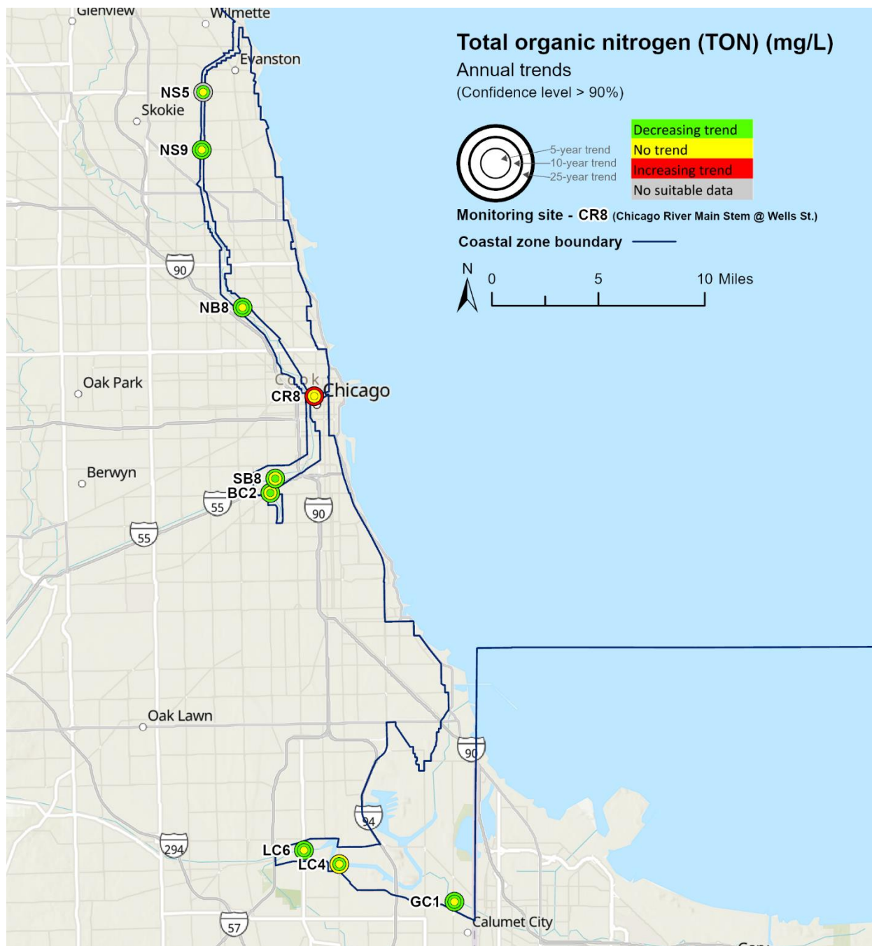
Figure C.26 Annual trends of total organic nitrogen
