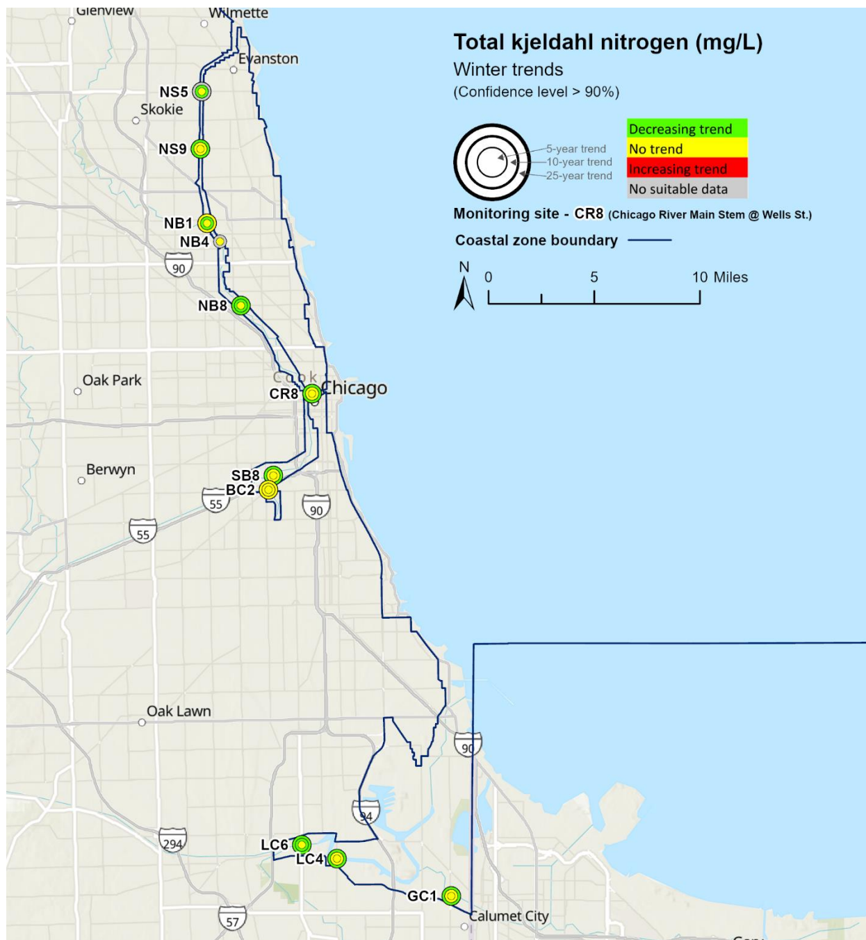
Winter trend slopes for total kjeldahl nitrogen (mg/L per year)
