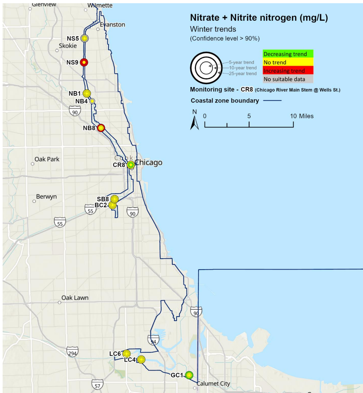
Winter trend slopes for nitrate + nitrite (mg/L per year)
