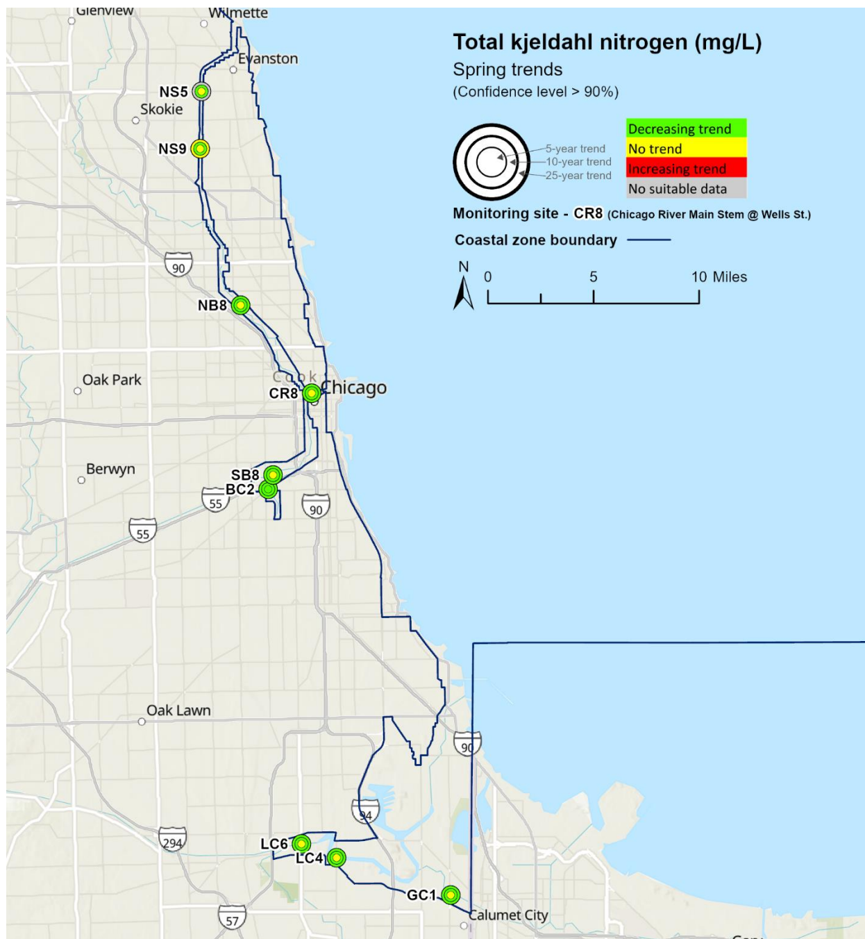
Spring trend slopes for total kjeldahl nitrogen (mg/L per year)
