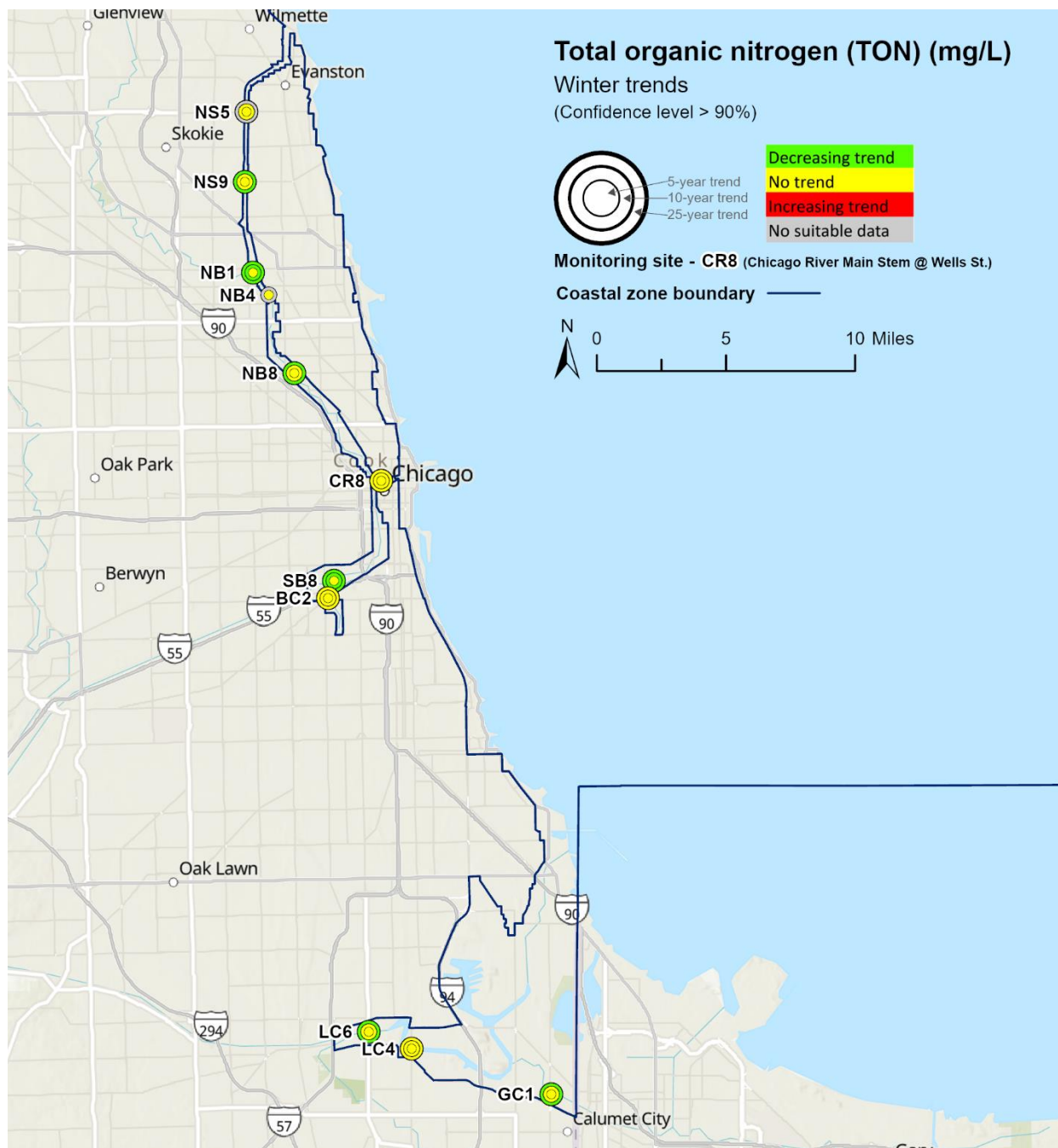
Winter trend slopes for total organic nitrogen (mg/L per year)
