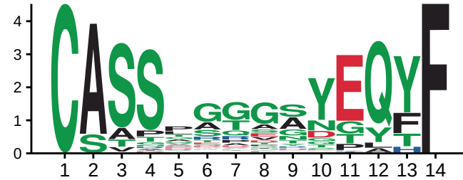
Input (178), CDR3b_14
