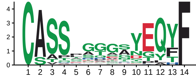
Input (174), CDR3b_14
