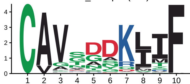
CDR3a_10 Input (256)
