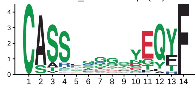
CDR3b_14 Baseline | P(VJ)
