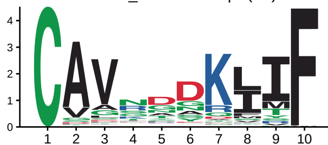
CDR3a_10 Baseline | P(VJ)
