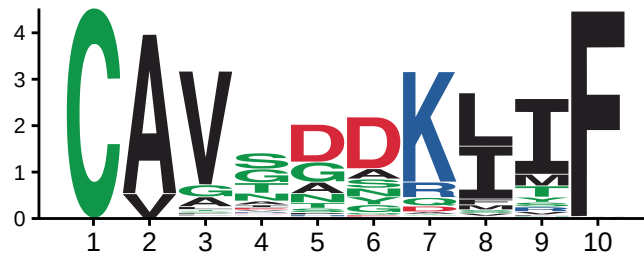
Input (256), CDR3a_10
