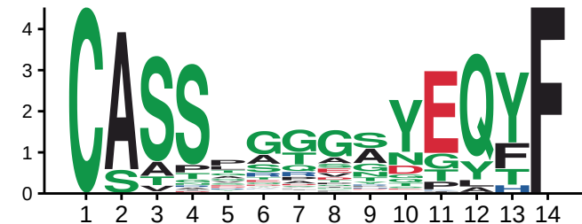
Input (178), CDR3b_14
