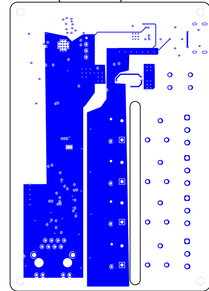
PWRD (Scale 2:3)
