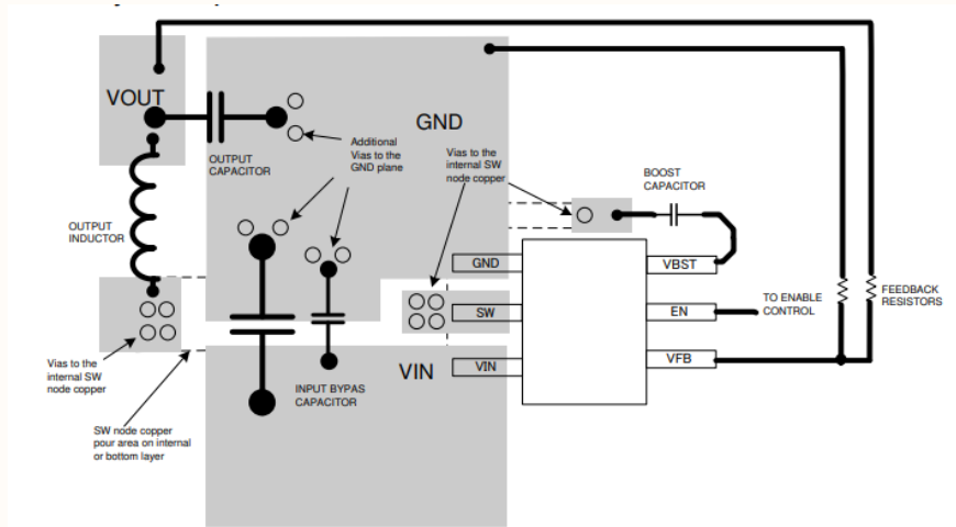
Figure 10-1. Board Layout
