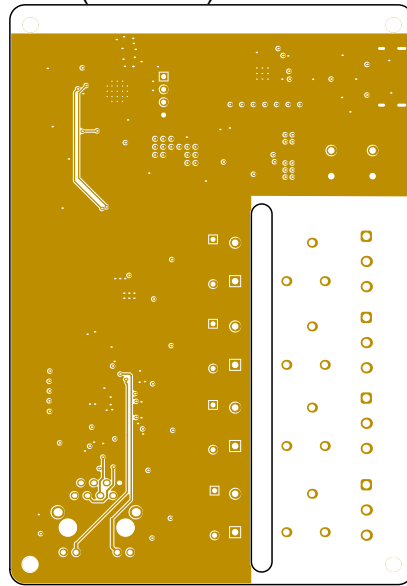
GND (Scale 2:3)
