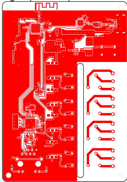
Signal (Scale 2:3)
