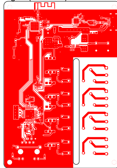
Signal (Scale 2:3)
