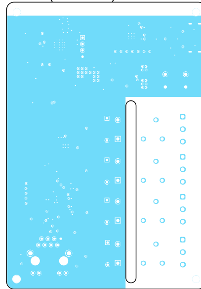
GND1 (Scale 2:3)
