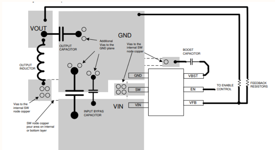
Figure 10-1. Board Layout
