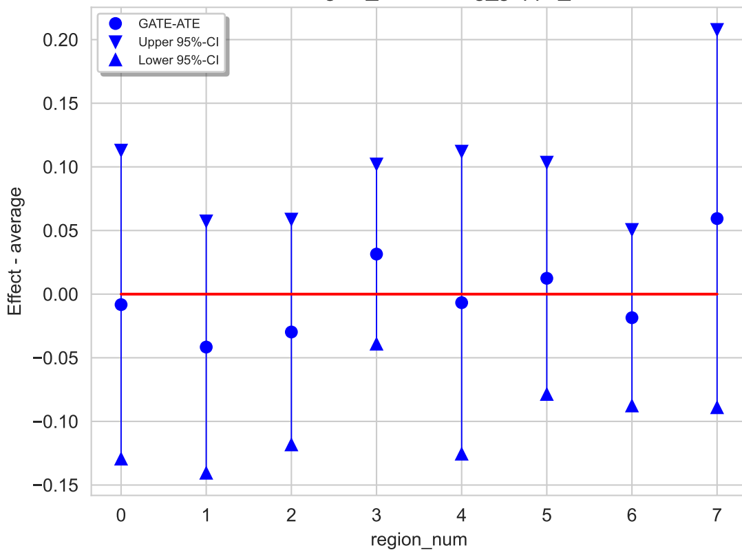
GATE - ATE region_num All log_gdppc_lc 2 vs 1
