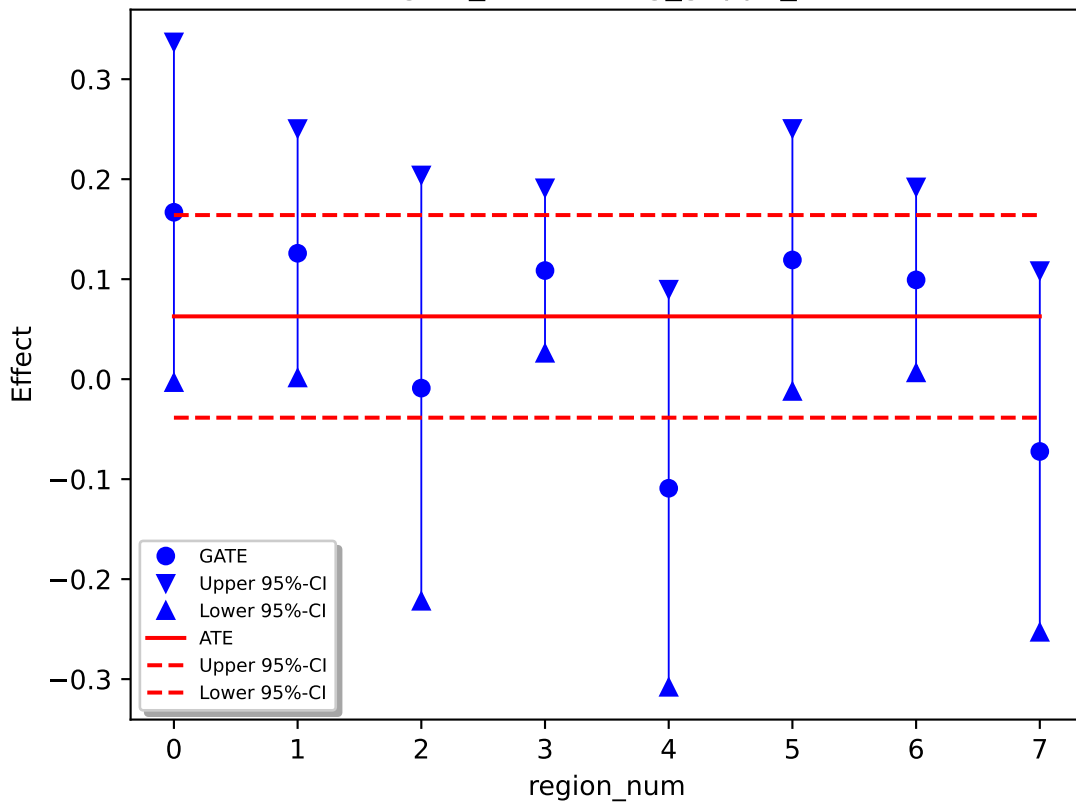
GATE region_num All log_gdppc_lc 2 vs 0
