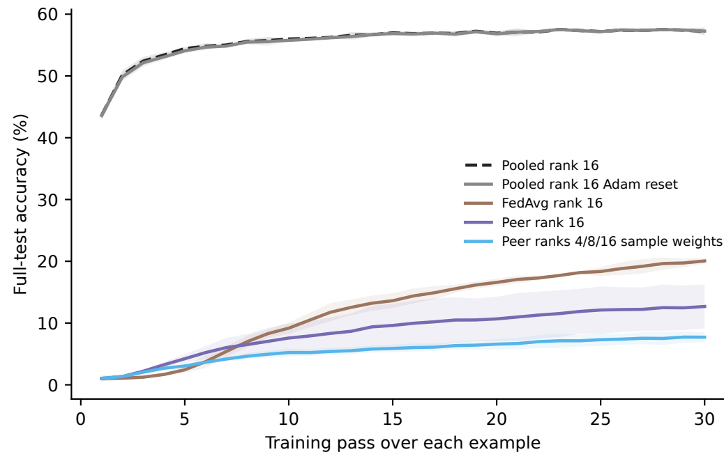
Pooled and communication controls
