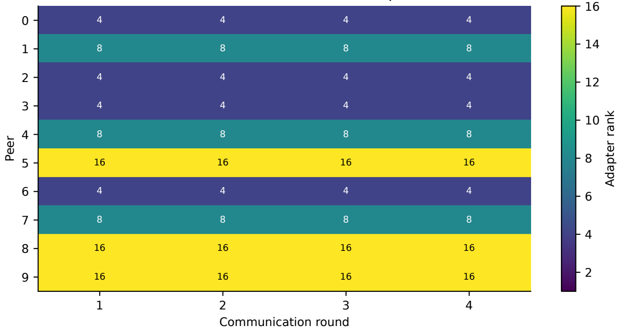
Fixed heterogeneous ranks, sample weights SST2 · smoke · seed 42; individual peers
