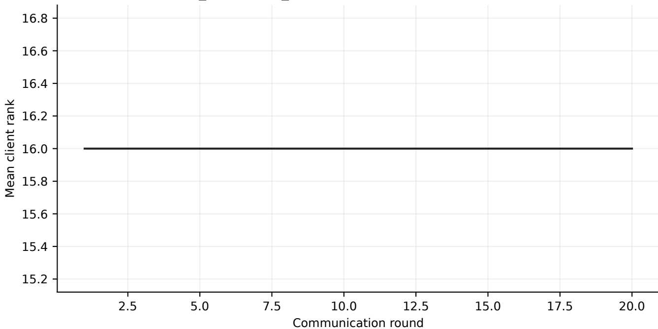
Dec-LoRA reimplementation, rank 16 SST2 · full_configured_budget · mean client rank \pm seed SD, n=5
