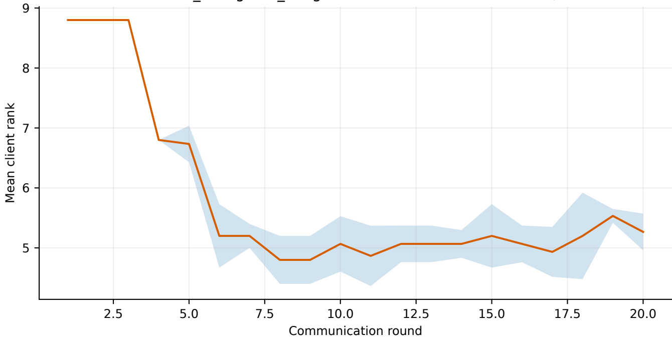
Adaptive ranks, sample weights SST2 · full_configured_budget · mean client rank \pm seed SD, n=3
