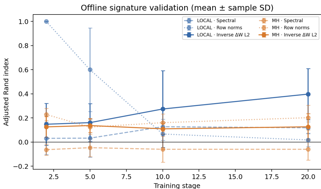
Figure 6: Historical local/MH offline signature validation. The stage-10 screen labels those methods weak-signal; adaptive-run descriptive scores are reported separately with the online discovery result.
