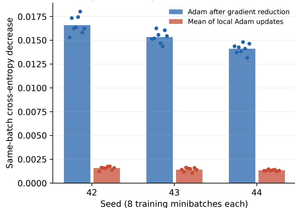
One optimizer step from shared initialization
