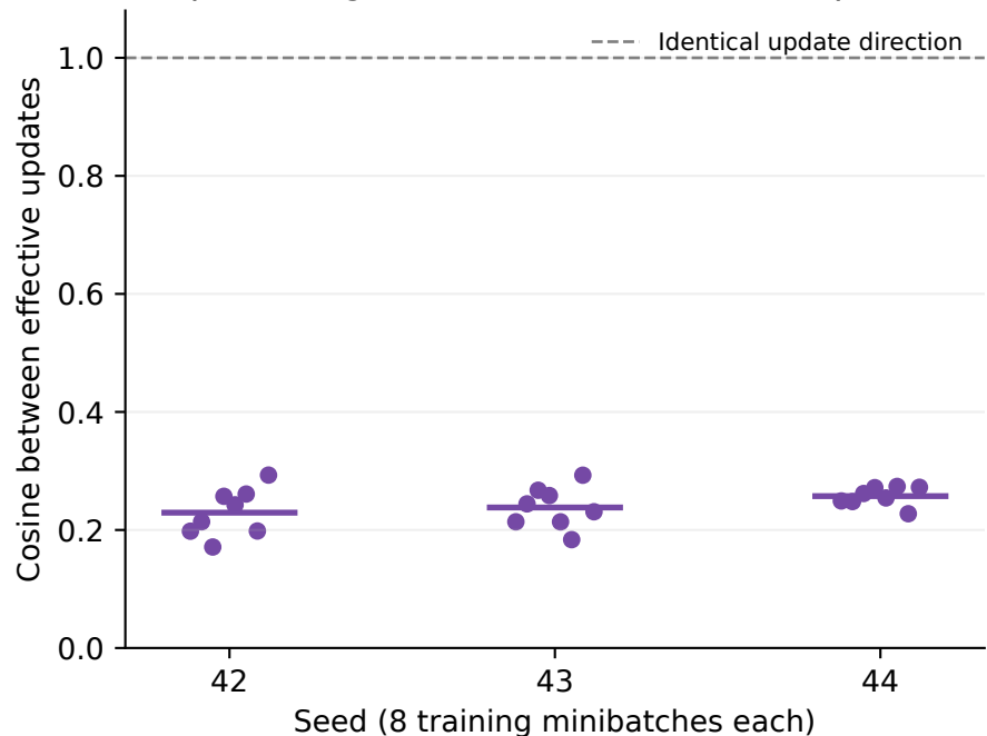
Equal raw gradients, different Adam updates
