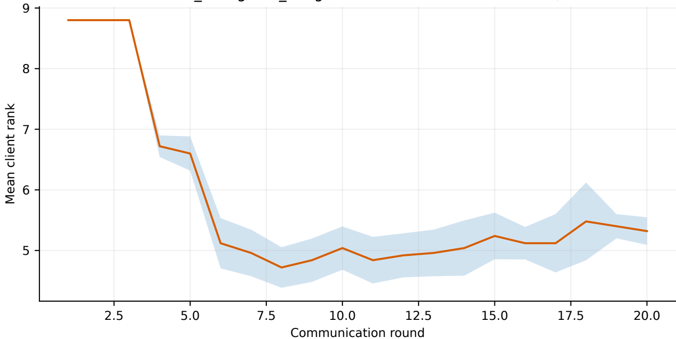
Adaptive ranks, sample weights SST2 · full_configured_budget · mean client rank \pm seed SD, n=5
