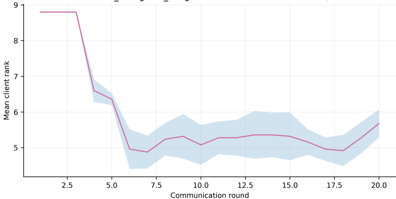
Adaptive ranks, uniform weights SST2 · full_configured_budget · mean client rank \pm seed SD, n=5
