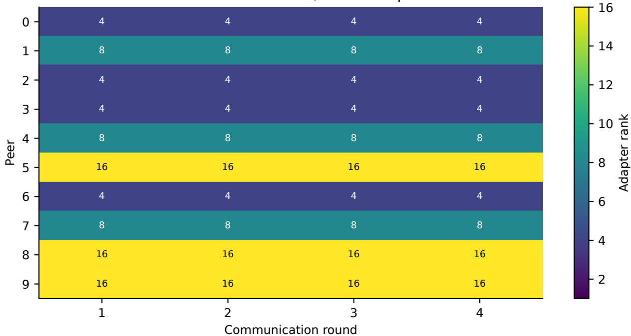
Fixed heterogeneous ranks, uniform weights SST2 · smoke · seed 42; individual peers
