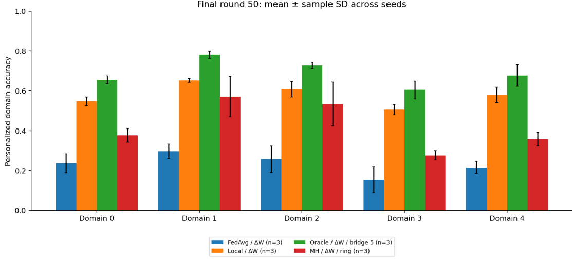
Figure 5: Uniform-rank per-domain personalized accuracy at the final round.
