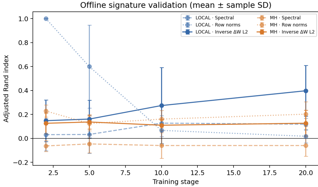
Figure 3: Offline signature validation. Early row-norm scores can be high for an individual stage, but performance is not stable across stages or seeds; the preregistered stage-10 screen labels all methods as weak-signal.
