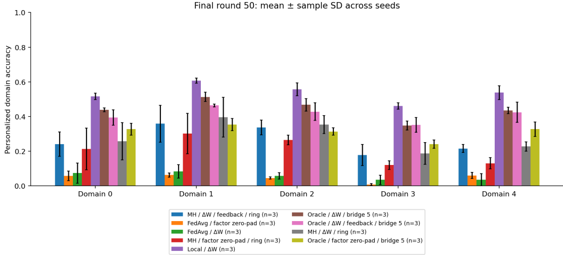
Figure 6: Heterogeneous-rank per-domain personalized accuracy at the final round.
