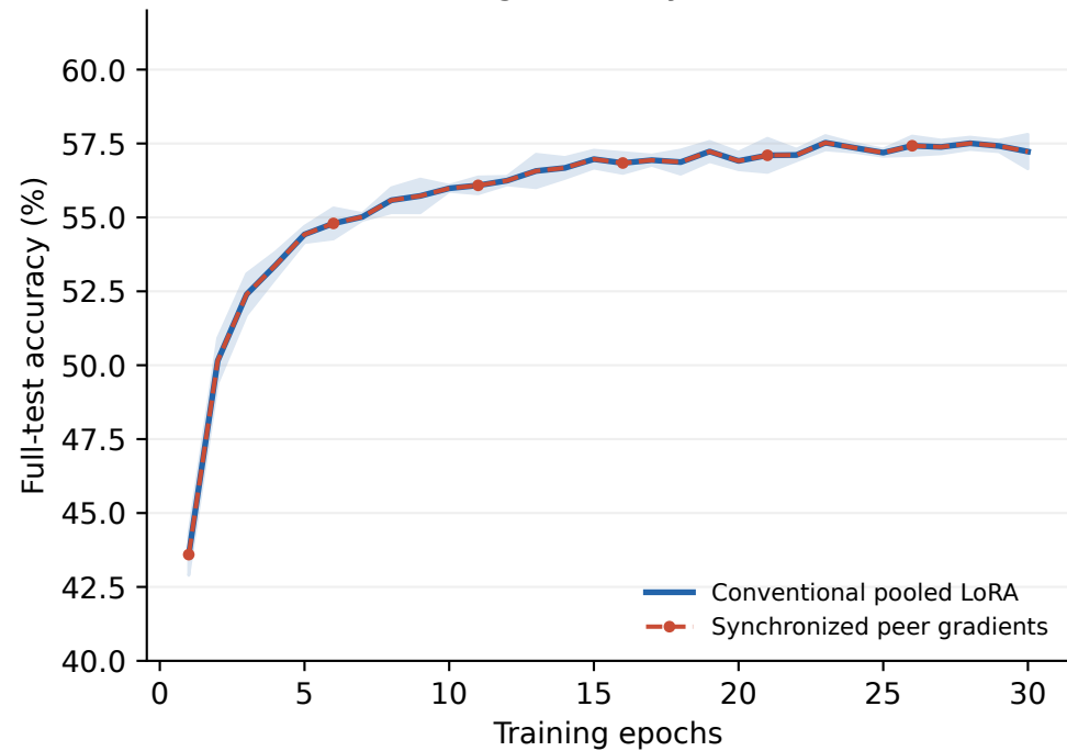
Matching accuracy (3 seeds)
