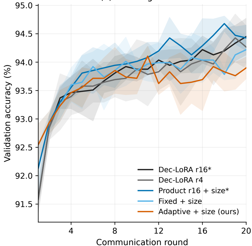
(a) Learning curves
