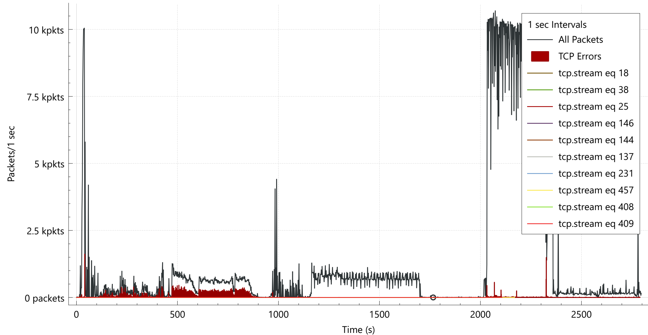
Wireshark I/O Graphs: traffic.pcapng
