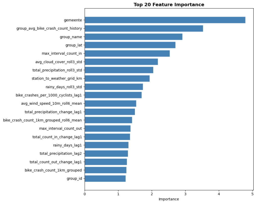
Figure 10: Top 20 feature importance scores from the final CatBoost model.
