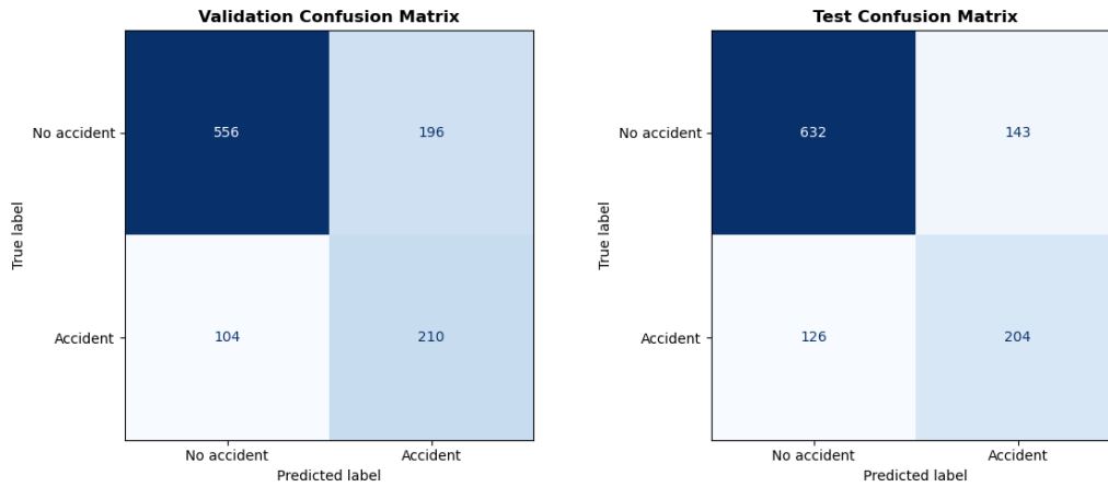
Figure 5: Confusion matrices for the final CatBoost model on the validation set (left) and test set (right).
