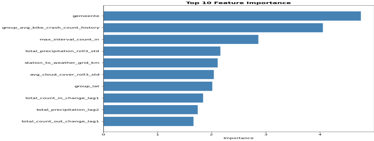
Figure 6: Top 10 feature importance scores from the final CatBoost model.
