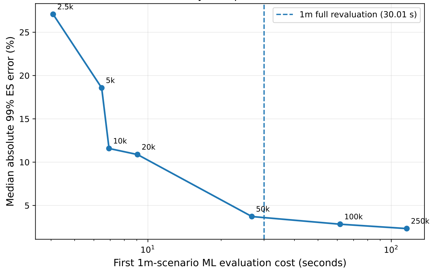
MLP Accuracy-Computation Trade-off
