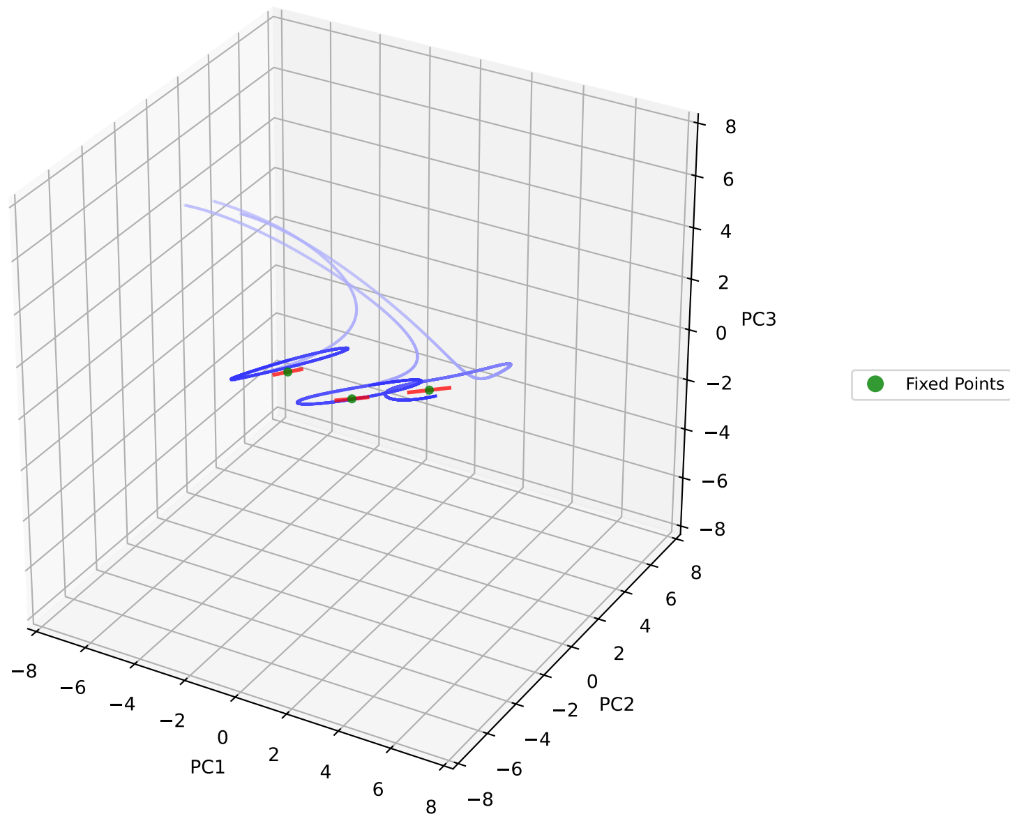
PCA of Network Trajectories and Fixed Points (Sparsity=0.00)
