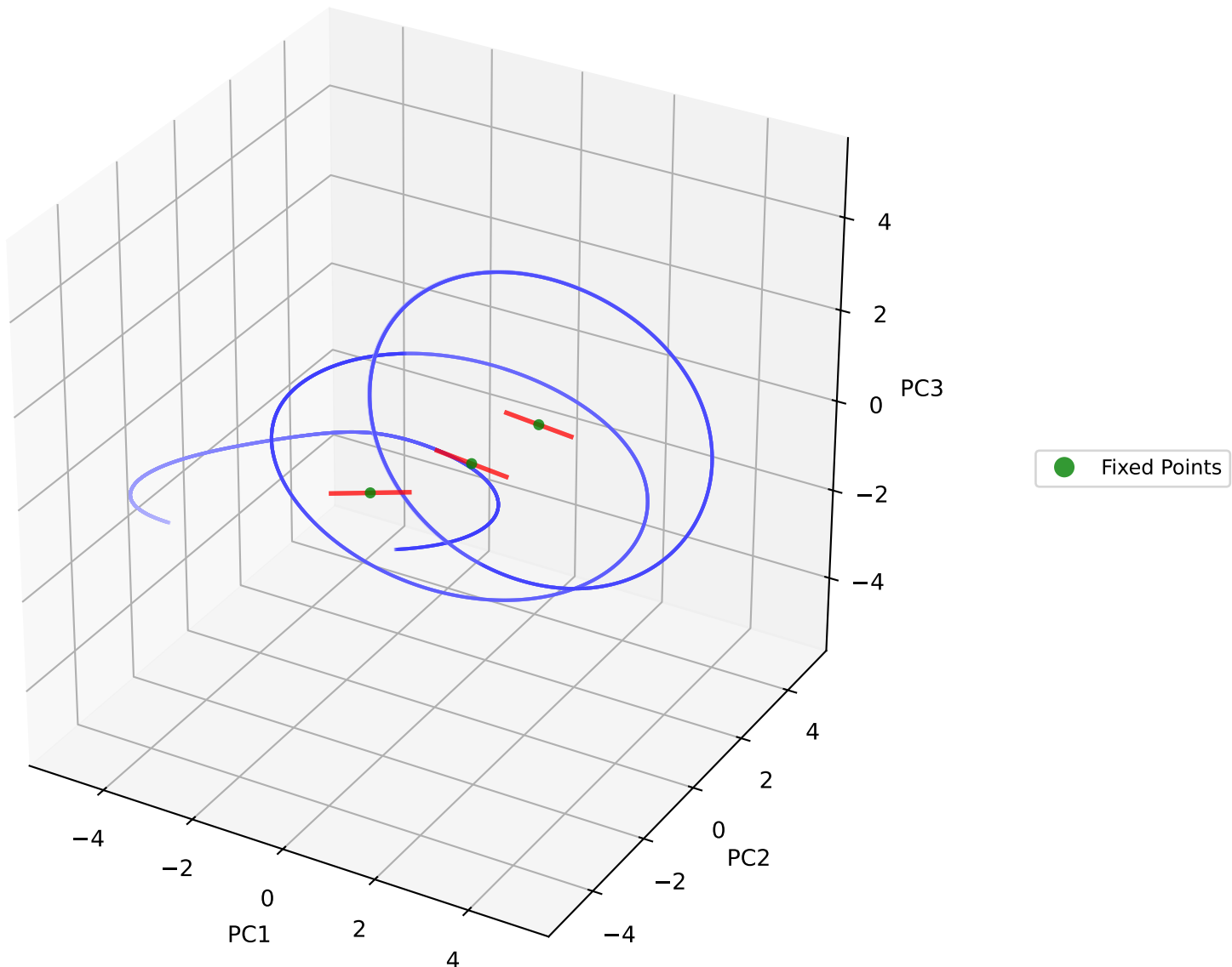
PCA of Network Trajectories and Fixed Points (skipping first 600 steps) (Sparsity=0.00)
