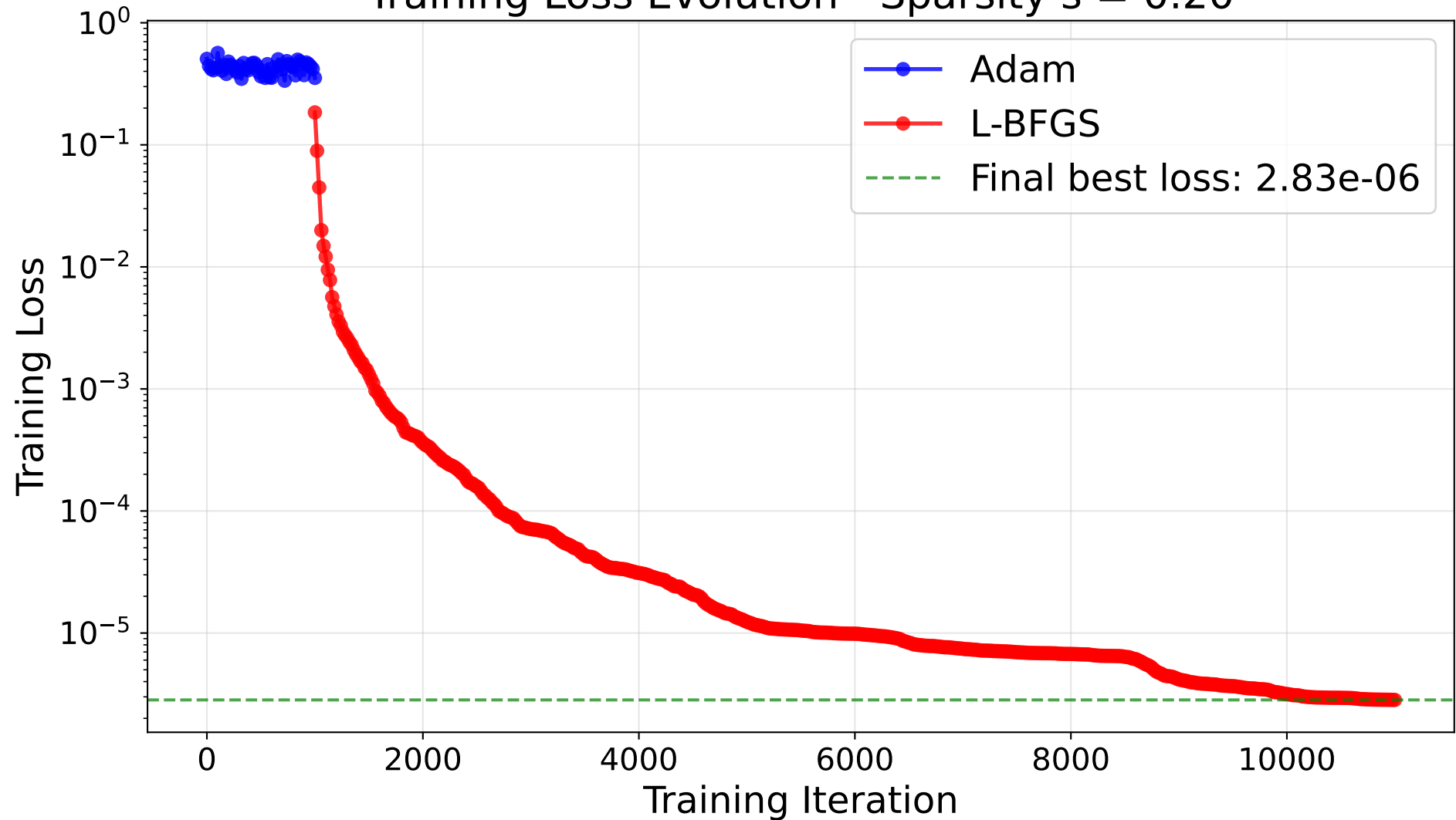
Training Loss Evolution - Sparsity s = 0.20
