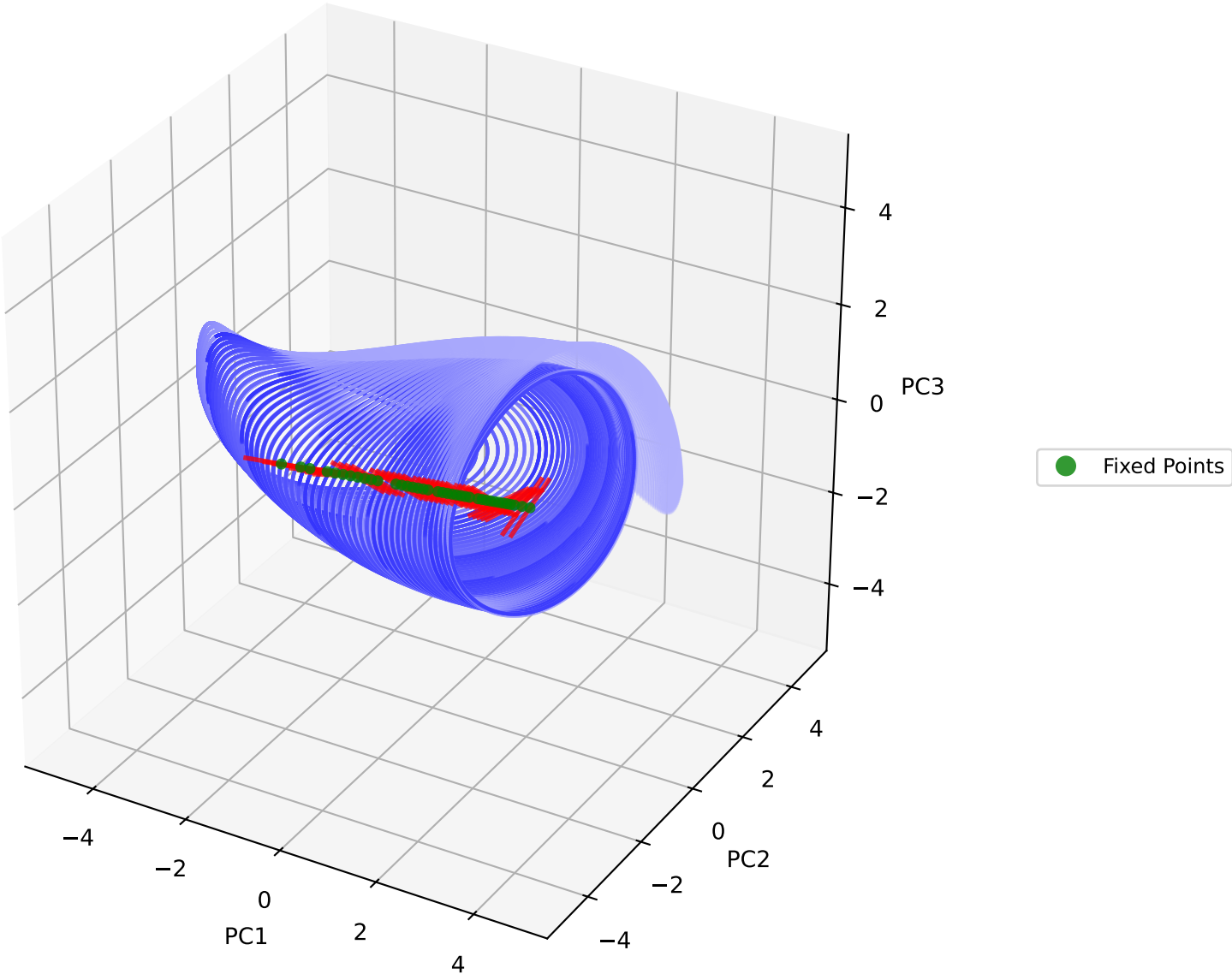
PCA of Network Trajectories and Fixed Points (tanh transformed) (Sparsity=0.00)
