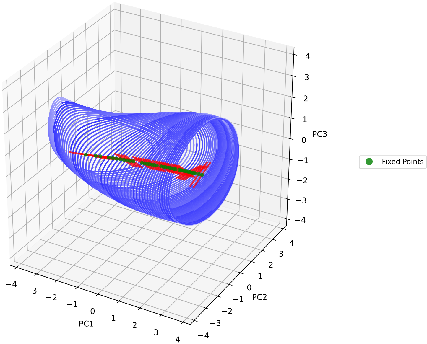
PCA of Network Trajectories and Fixed Points (skipping first 600 steps) (tanh transformed) (Sparsity=0.00)
