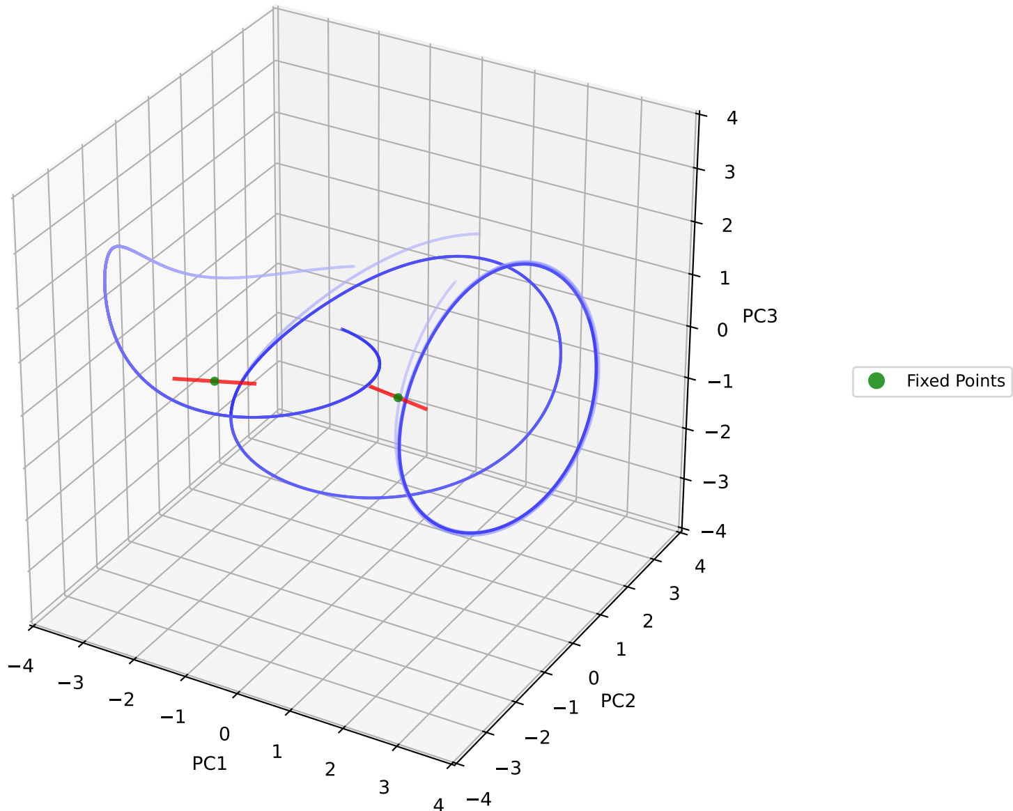
PCA of Network Trajectories and Fixed Points (skipping first 200 steps) (tanh transformed) (Sparsity=0.00)
