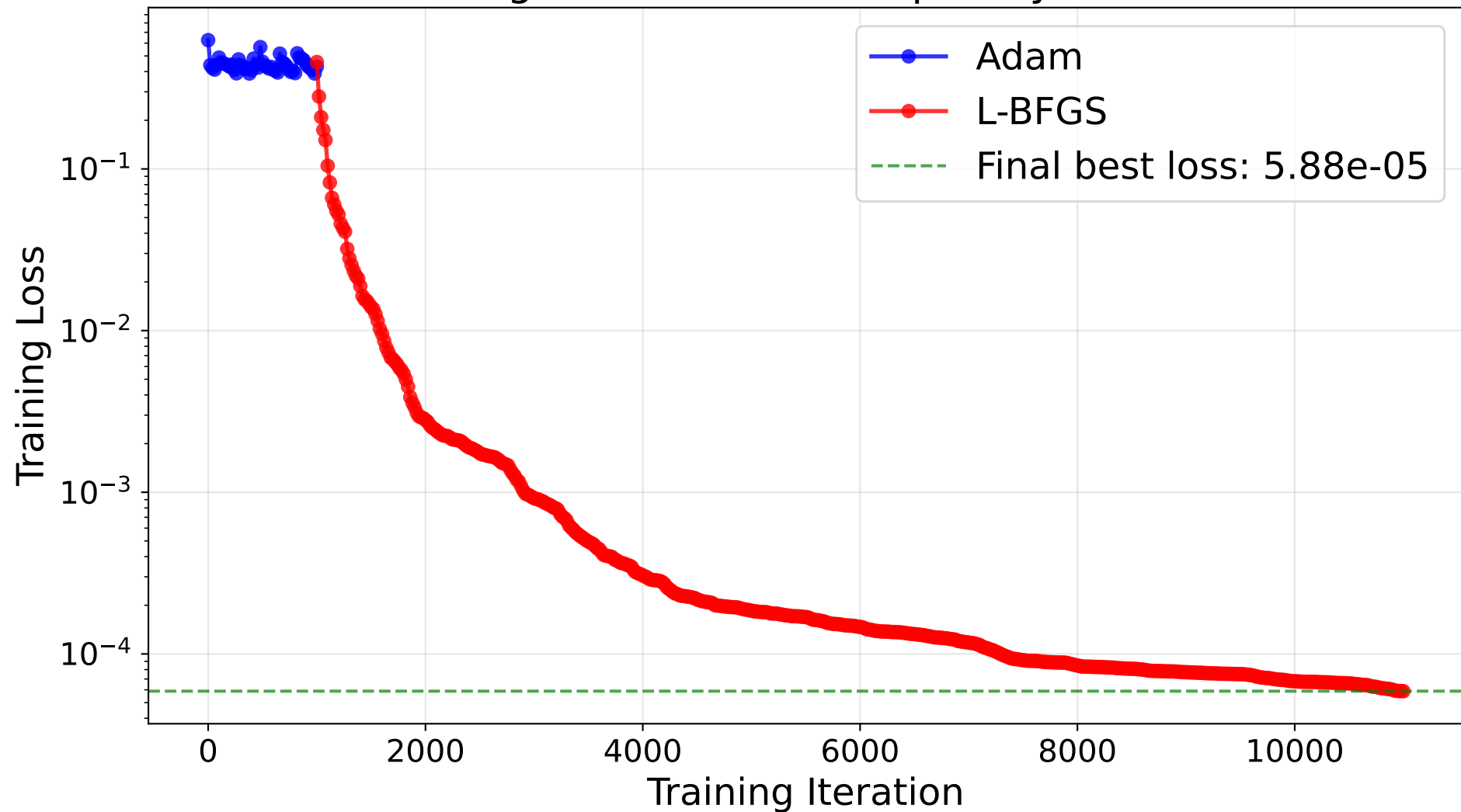
Training Loss Evolution - Sparsity s = 0.40
