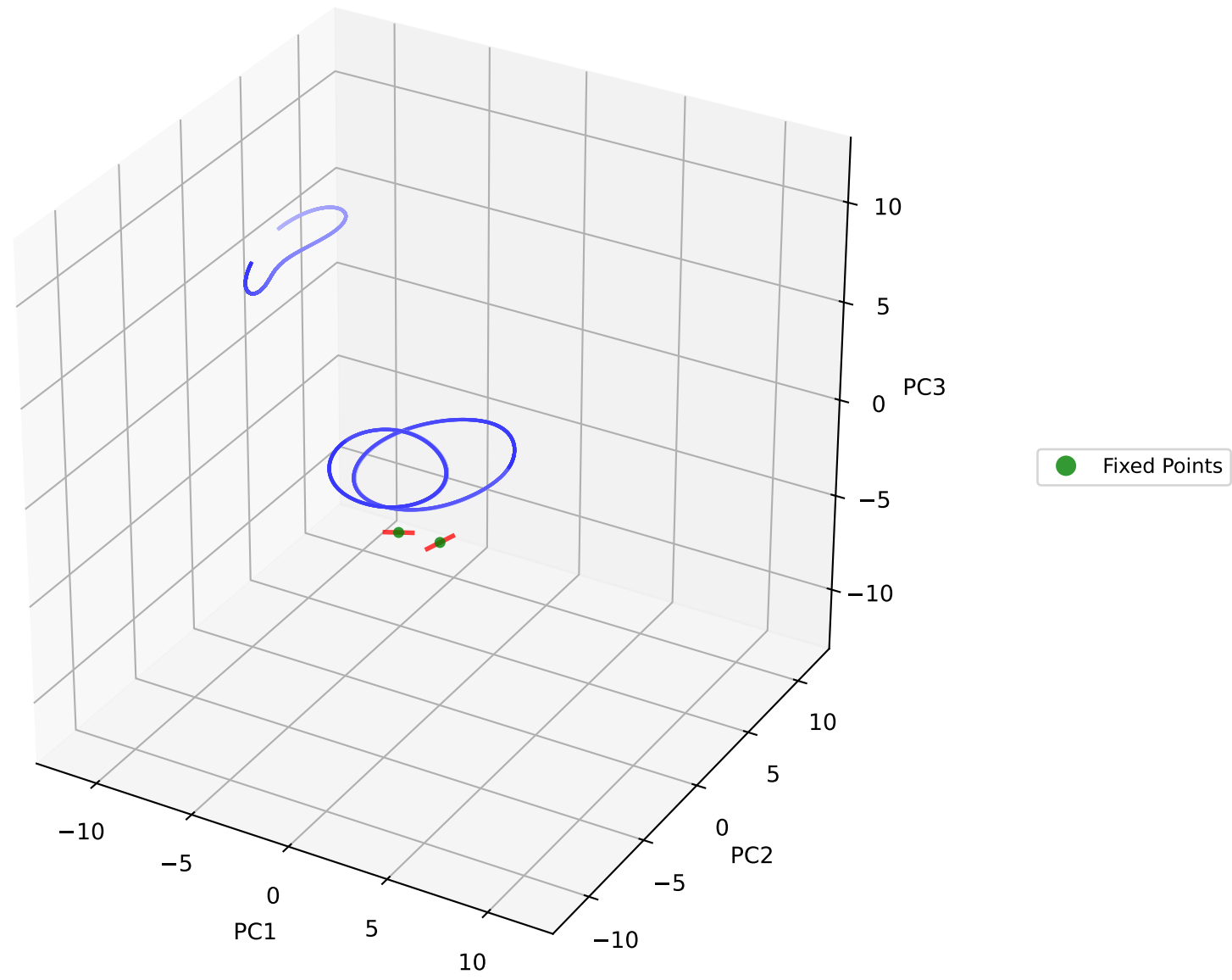
PCA of Network Trajectories and Fixed Points (skipping first 600 steps) (tanh transformed) (Sparsity=0.00)
