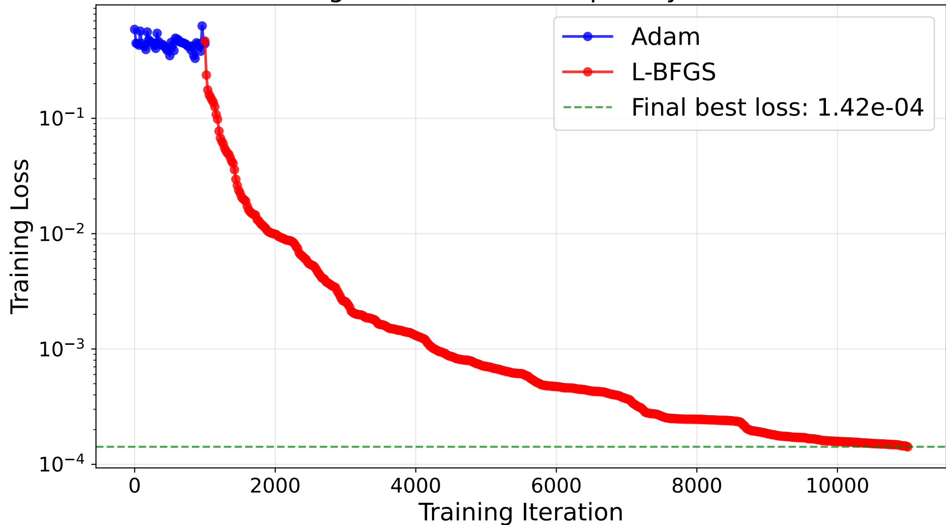
Training Loss Evolution - Sparsity s = 0.60
