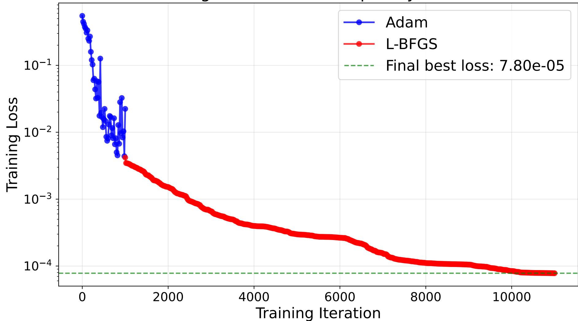
Training Loss Evolution - Sparsity s = 0.80
