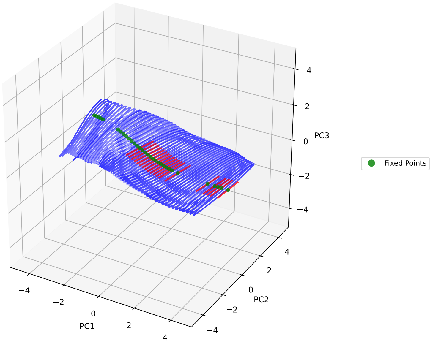
PCA of Network Trajectories and Fixed Points (skipping first 400 steps) (Sparsity=0.00)
